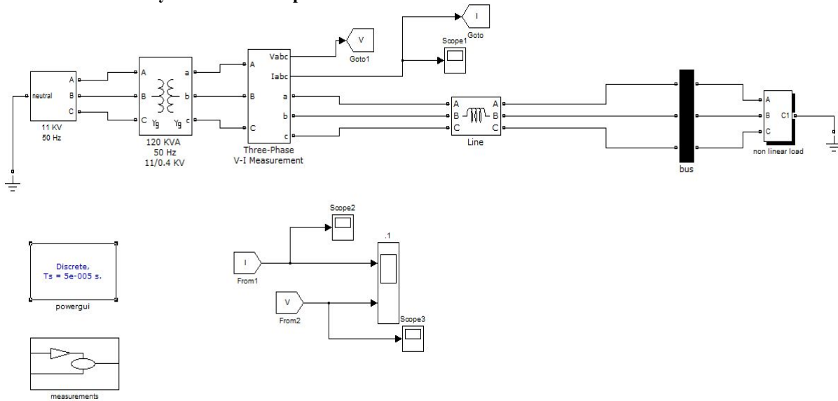
Fig.4. Simulation model of system without SAPF
