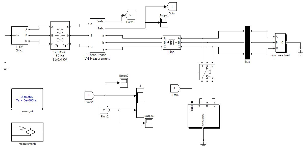
Fig.8 Simulation model of system with SAPF
