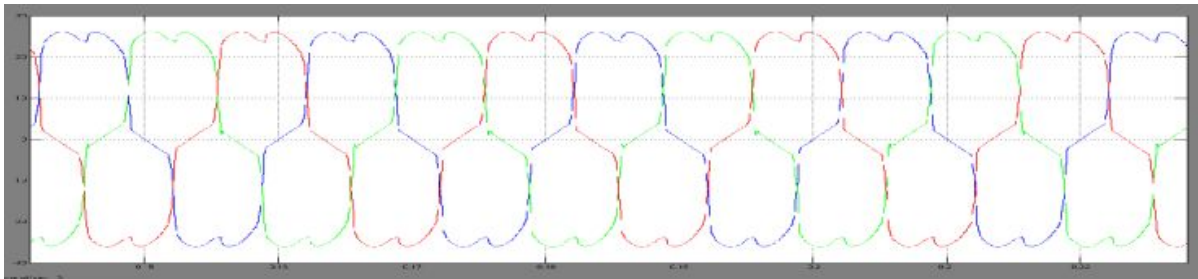
Fig.5 Voltage and current waveform without filter
